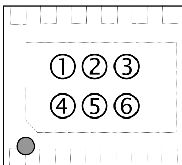
DFN(PLP)2730-12 Part Markings
