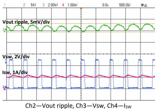
Output Ripple and SW at 1A load Vin=5V / Vout=1.2V
